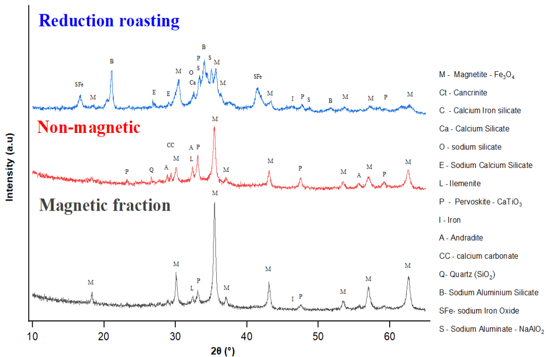
Figure 4. XRD patterns of reduced BR (at 500 °C, 20 wt% NaOH, 30 min reduction time), magnetic and non-magnetic residues after water leaching, and wet-magnetic separation.
