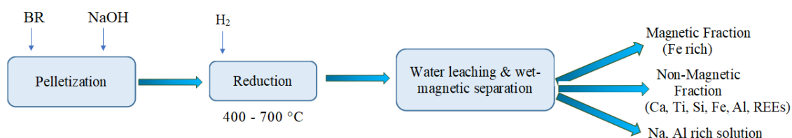
Figure 1. Flow sheet of experimental procedure followed in this work.
